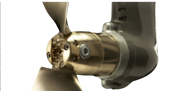
Engine (Diesel) 38 HP, two blade folding propeller
