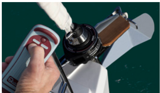
Anchor windlass, electrical with remote control
